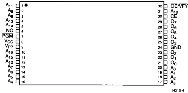
TSOP Top View
